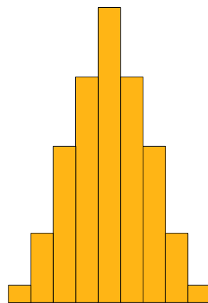
Histograma HSPE
